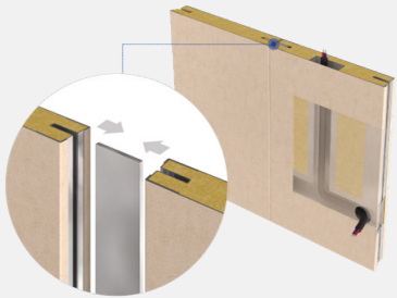
Bar Joint Type
