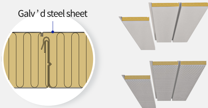
Ceiling Panel (No-Gap / No-Gap Perforated Type)
