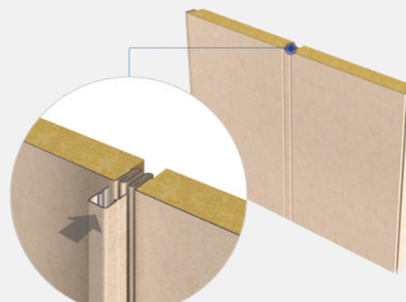
C-Clip Joint Type
