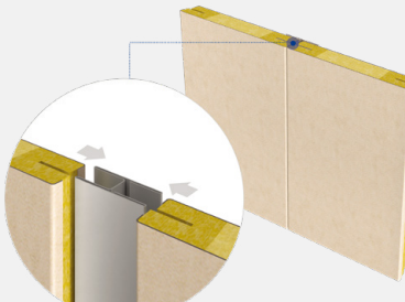
H Joint Type
