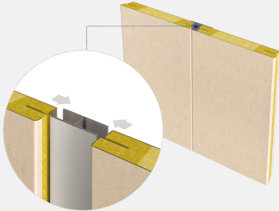
Wall Panel (H Joint Type)
