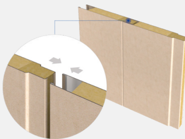
Insert Joint Type
